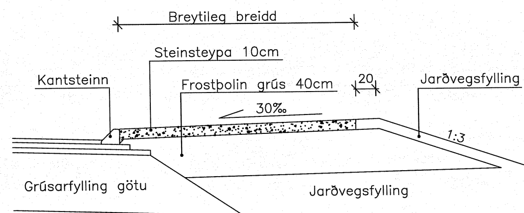
GANGSTÉTT, LÁGMARKSBAKFYLLING
