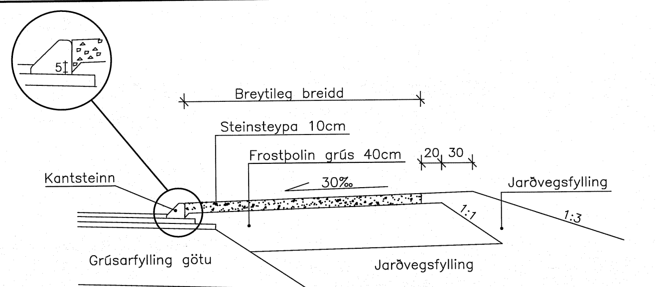
GANGSTÉTT, BAKFYLLING \geq 50 cm.
