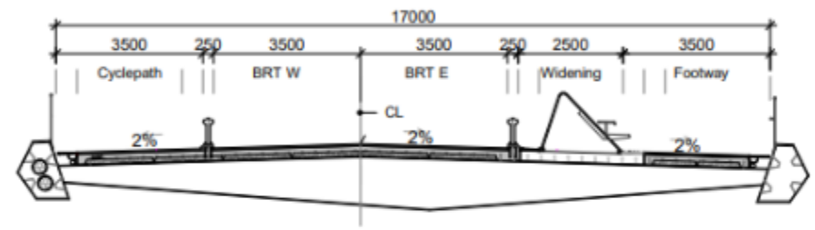
4 General cross section - Span 1 : 100
